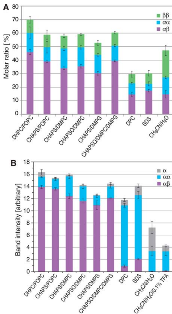
Figure 2. Relative quantities of accumulated \alpha Ib/ \beta 3 TM species as a function of membrane mimic. (A) Dimeric species obtained with GB3-off7- \alpha Ib(Ala963Cys) and GB3- \beta 3(Gly690Cys) proteins. The size of each color-coded bar denotes its molar ratio among \alpha , \beta , \alpha\alpha , \beta\beta , and \alpha\beta species. For visual clarity, explicit bars were omitted for \alpha and \beta . (B) Species obtained with GB3- \alpha Ib(Ala963Cys) and \beta 3(Gly690Cys) proteins. The size of each color-coded bar approximates the mass distribution of GB3-tagged \alpha Ib among \alpha , \alpha\alpha , and \alpha\beta species. Figure S4B depicts the corresponding distribution for \beta 3. In all experiments, the molar ratio of \alpha Ib: \beta 3:short-chain lipid/detergent:long-chain lipid was 1:1:2000:600 with protein concentrations of 10 \mu\text{M} . Error bars denote the standard error of the mean of three experiments. Abbreviations are DHPC (1,2-dihexanoyl- sn -glycero-3-phosphocholine), POPC (1-palmitoyl-2-oleoyl- sn -glycero-3-phosphoglycerol), CHAPS (3-[(cholamidopropyl) dimethyl-ammonio]-1-propane sulfonate), DMPC (1,2-dimyristoyl- sn -glycero-3-phosphocholine), CHAPSO (3-[(3-cholamidopropyl)dimethylammonio]-2-hydroxy-1-propanesulfonate), DMPG (1,2-dimyristoyl- sn -glycero-3-phosphoglycerol), DPC (dodecylphosphocholine), SDS (sodium dodecyl sulfate), and TFA (trifluoroacetic acid).
