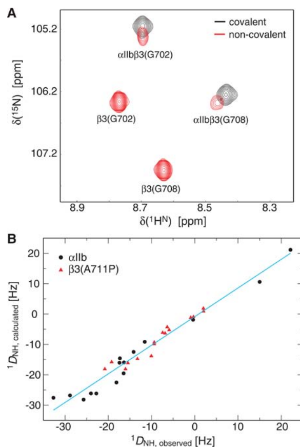
Figure 4. Structural properties of the covalently associated integrin \alpha\text{IIb}:\beta 3 TM complex. (A) Comparison of H–N correlation spectra of covalently and noncovalently associated \alpha\text{IIb}:\beta 3 TM domains. ^1\text{H}/^{14}\text{N} -labeled \alpha\text{IIb} and ^2\text{H}/^{15}\text{N} - \beta 3 TM peptides or ^2\text{H}/^{15}\text{N} -labeled, covalently linked \alpha\text{IIb}(\text{Ala}963\text{Cys})-\beta 3(\text{Gly}690\text{Cys}) peptides were reconstituted at concentrations of 0.1 mM each in 200 mM DHPC, 60 mM POPC, 25 mM HEPES-NaOH, pH 7.4. Spectra were recorded at 700 MHz and 28 ^\circ\text{C} . (B) Residual dipolar coupling (RDC) of the \alpha\text{IIb}(\text{A}963\text{C})-\beta 3(\text{G}690\text{C}) cross-linked integrin \alpha\text{IIb}:\beta 3(\text{A}711\text{P}) TM complex at 40 ^\circ\text{C} . Measured ^1D_{\text{NH}} couplings were fitted to the monomeric \alpha\text{IIb} and \beta 3(\text{A}711\text{P}/\text{K}716\text{A}) TM structures (PDB ID 2K1A and 2L91), 17,25 respectively, to back-calculate ^1D_{\text{NH}} ( R = 0.980 ).
