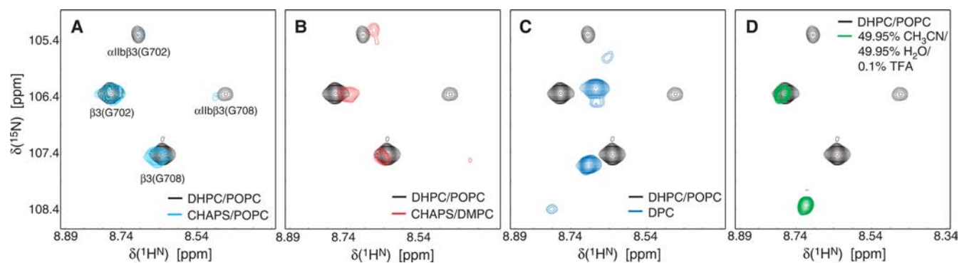
Figure 3. H–N correlation spectra of noncovalently associated integrin ^1\text{H}/^{14}\text{N} -labeled \alpha\text{IIb} and ^2\text{H}/^{15}\text{N} -labeled \beta 3 TM domains as a function of membrane mimic. (A) Comparison of DHPC/POPC with CHAPS/POPC bicelles at relative contour levels of 1:0.70. In the slow exchange regime, monomeric and heterodimeric resonances are observable 4,10 and were observed here for the ^{15}\text{N} -labeled \beta 3 subunit as indicated. (B) Comparison of DHPC/POPC with CHAPS/DMPC bicelles at relative contour levels of 1:0.49. (C) Comparison of DHPC/POPC bicelles with DPC micelles at relative contour levels of 1:0.84. (D) Comparison of DHPC/POPC bicelles with 49.95% \text{CH}_3\text{CN}/49.95\% \text{H}_2\text{O}/0.1\% \text{TFA} at relative contour levels of 1:2.52. Peptide concentrations of 0.1 mM were used in all samples with a molar ratio of \alpha\text{IIb}:\beta 3 :short-chain lipid/detergent:long-chain lipid of 1:1:2000:600. Spectra were recorded using ^2\text{H}/^{15}\text{N} -labeled peptides in 25 mM HEPES-NaOH, pH 7.4 solution at a ^1\text{H} frequency of 700 MHz at 28 ^\circ\text{C} .
